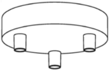
KRM573FGOTERM 3 hole ø 120mm H 25mm
